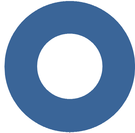
Calls Per Species For BROADLANDS
