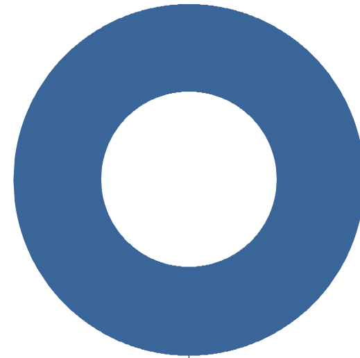
Calls Per Species For PESOTUM
