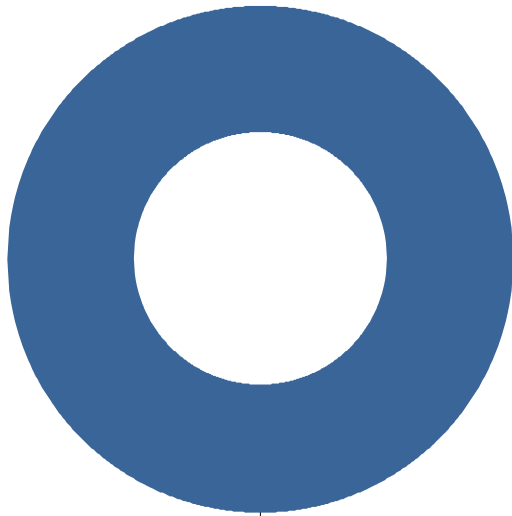
Call Types For PESOTUM
