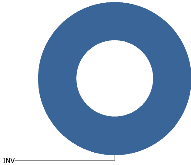
Call Types For MAHOMET
